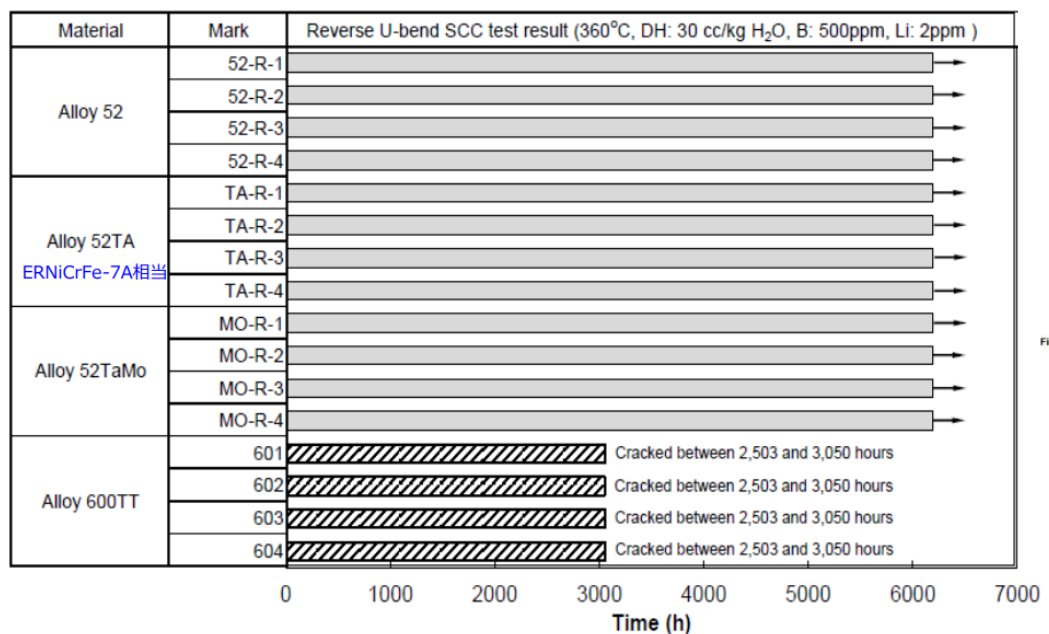
Figure 12: SCC initiation test results
