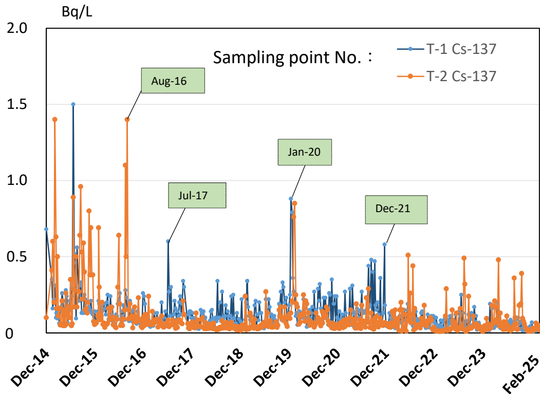
Concentration ranges of Cs-137 in sea-water near the Fukushima Daiichi NPS surveyed by TEPCO
