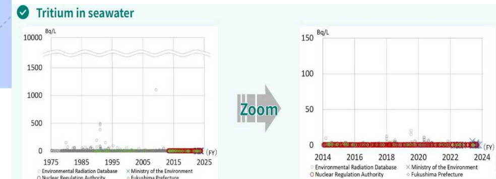
Comparison with previous tritium concentration in Japan
