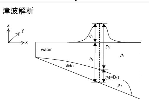
Fig. 3. Initial and boundary conditions of the two-layer model.
