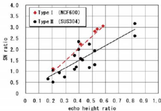
Fig. 9 Relationship between echo height ratio and SN ratio in type I and type II specimens
