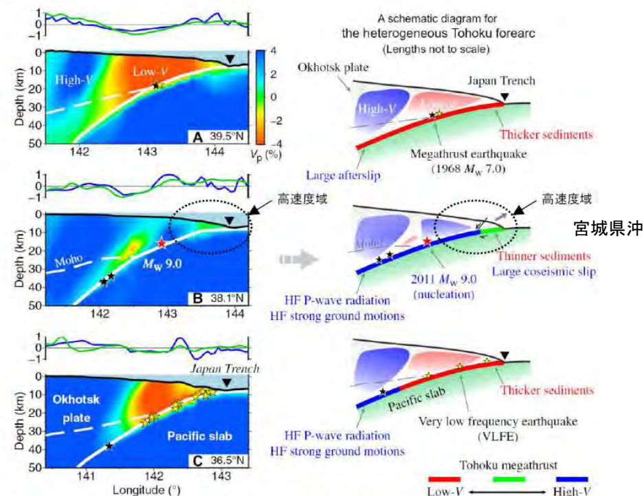
Fig. 5. Vertical cross sections of V_p tomography (left) and corresponding cartoons (right). The east-west vertical cross sections are along the three profiles shown in Fig. 1C. The normalized residual topography (blue line) and gravity (green line) along each profile are shown atop each cross section. The red and blue colors in (A) to (C) denote low and high V_p perturbations, respectively, whose scale is shown beside (A). The white bold and dashed lines in (A) to (C) denote the UBPs and the forearc Moho, respectively. The red star denotes the mainshock hypocenter of the 2011 Tohoku-oki earthquake ( M_w 9.0). The black and yellow stars indicate other megathrust earthquakes ( M_w 7.0 to 8.0) during 1917 to 2017 and the VLFs (24) within a 40-km width of each profile, respectively. Note that the hypocenters of the VLFs and the megathrust earthquakes are set on the UBPs, because their accurate focal depths are unclear for most of them. The reverse triangle denotes the Japan Trench axis. HF, high-frequency. In the right panels, the red, green, and blue lines denote low-, normal-, and high- V_p anomalies atop the subducting Pacific plate, respectively, according to the tomographic results of this study. The gray dashed line denotes the forearc Moho.
