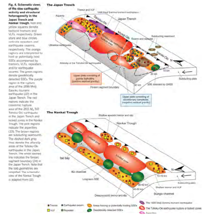
Fig. 4. Schematic views of the slow earthquake activity and structural heterogeneity in the Japan Trench and Nankai Trough. Red and yellow squares denote tectonic tremors and VLFs, respectively. Green stars and blue circles indicate repeaters and earthquake swarms, respectively. The orange regions are interpreted to host or potentially host SSEs accompanied by tremors, VLFs, repeaters, and/or earthquake swarms. The green regions denote geospatially detected SSEs. The purple region is the rupture area of the 1996 M w 7.1 Sanriku tsunami earthquake (22) in the Japan Trench. The red regions indicate the coseismic rupture area of the 2011 M w 9.0 Tohoku-Oki earthquake in the Japan Trench and locked zones in the Nankai Trough. The pink regions indicate the afterslip areas of the Tohoku-Oki earthquake in the Japan Trench. The white dashed line indicates the forearc segment boundary (24) in the Japan Trench. Note that the slab geometries are simplified. The schematic view of the Nankai Trough is adapted from (22).
