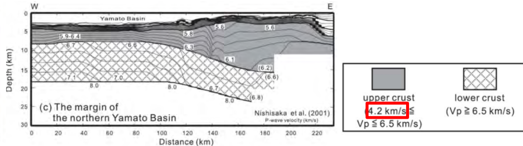
Sato et al. (2006) (73) に一部加筆
