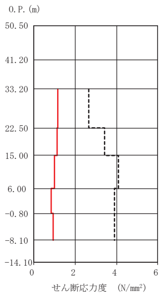
OW-1
