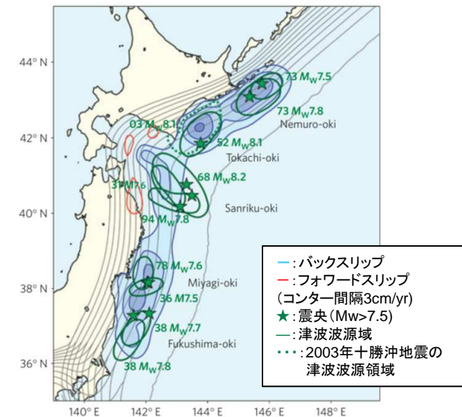
Figure 4 | Comparison of slip-deficit zones and tsunami source regions.
