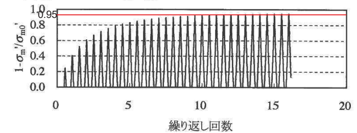
過剰間隙水圧比(=1- \sigma'_m/\sigma_{m0} )時刻歴
