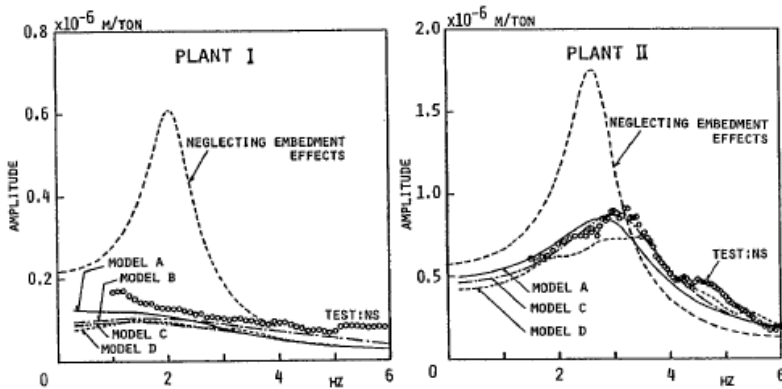
Fig. 1 Embedded Structures
