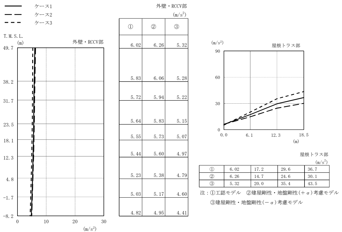
(b) Ss-2
