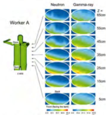
In the JCO criticality accident A. Endo and Y. Yamaguchi, Radiation Res. (2003)
