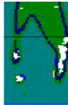
In the overexposure case with gamma radiography FCA DaSaliva et al., J. Radiat.Prot. (2005)
