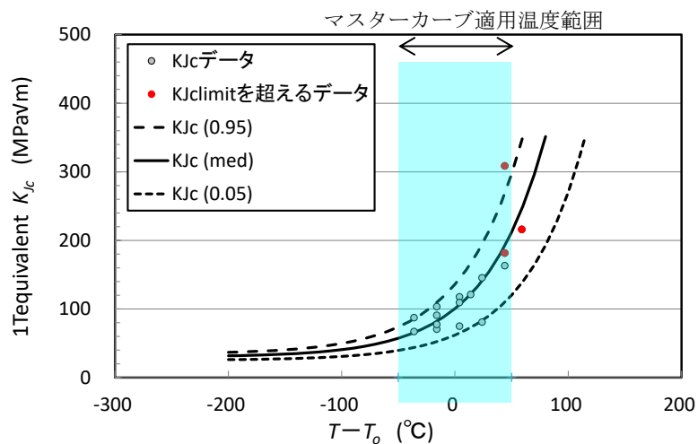
(c) 鍛鋼品 No. 3 (照射量 2.7 \times 10^{19} n/cm 2 , T_0 = -64^\circ\text{C} )
