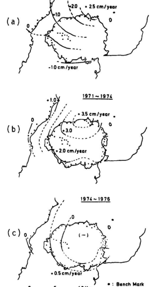
Fig. 3. Distributions of the rates of vertical displacements around Sakurajima Volcano in each period shown in Fig. 2.
