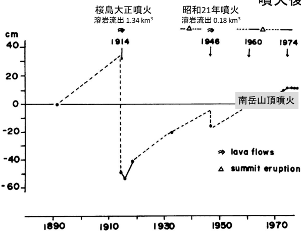
Fig. 1. Change of height of BM.2474 referred to BM.2469 shown in Fig. 2.
