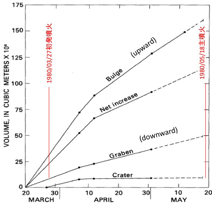
Figure 71.—Volume changes of Mount St. Helens, March 20 to May 18, 1980. Dashed lines are estimates (where features are not discernible on photos due to cloud cover).
