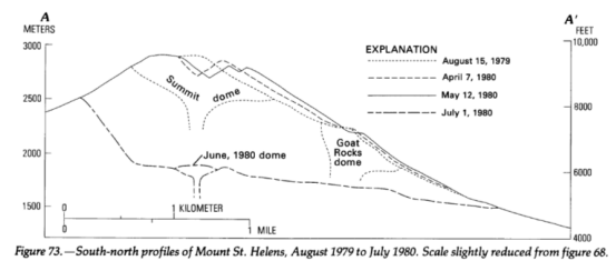
Figure 73.—South-north profiles of Mount St. Helens, August 1979 to July 1980. Scale slightly reduced from figure 68.
