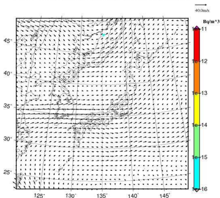
Cs-137 concentration at 3000m JST= 2017-09-06_12h00m
