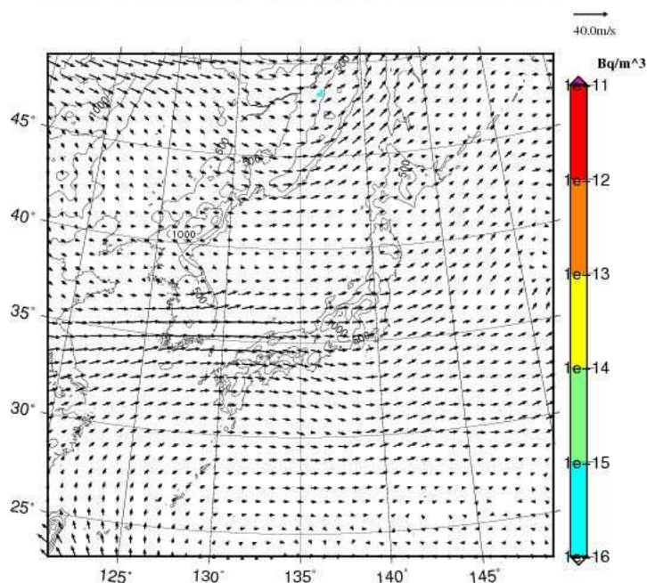
Cs-137 concentration at 3000m JST= 2017-09-06_15h00m
