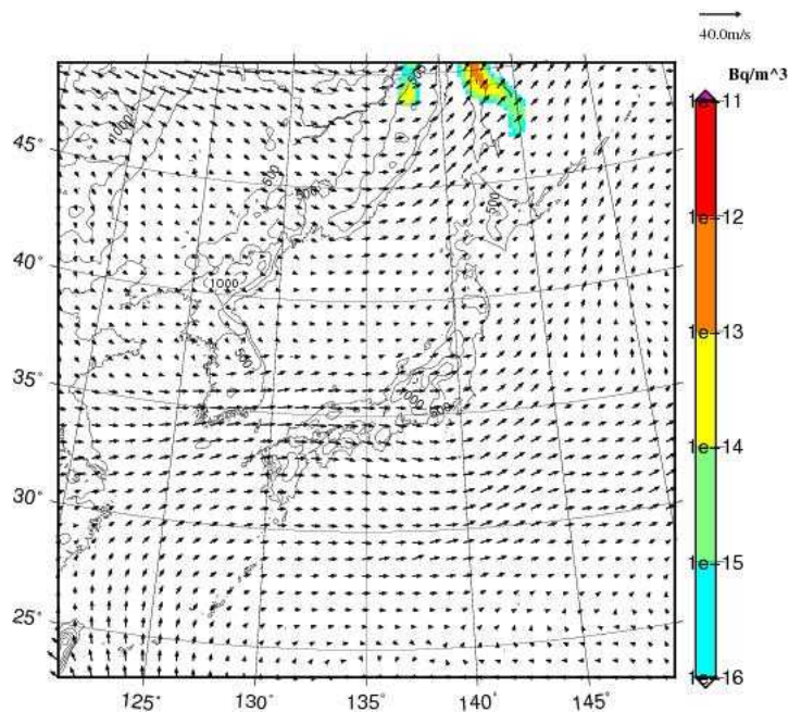
Xe-133 concentration at 2000m JST= 2017-09-06_18h00m
