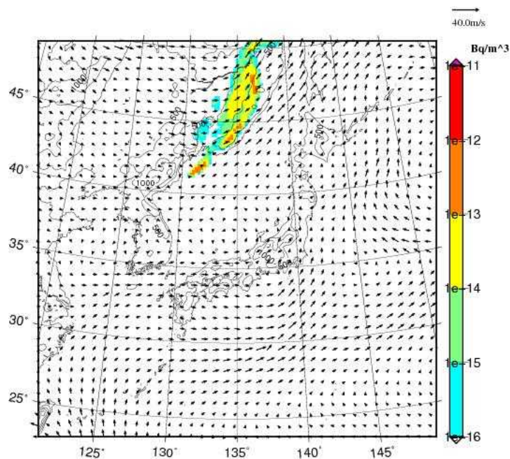
I-131 concentration at 1000m JST= 2017-09-06_12h00m
