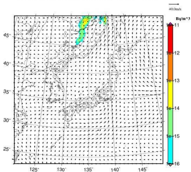
I-131 concentration at surface JST= 2017-09-06_12h00m
