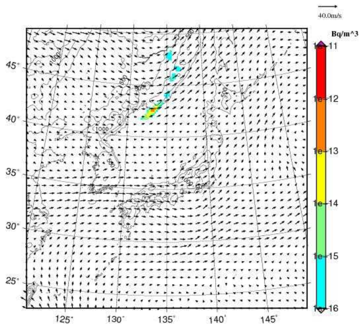
Cs-137 concentration at 2000m JST= 2017-09-06_12h00m
