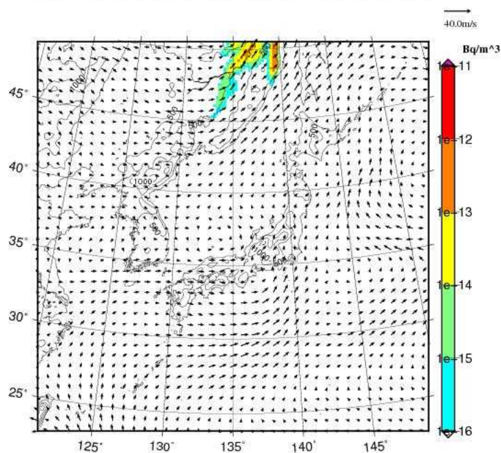
Cs-137 concentration at 1000m JST= 2017-09-06_09h00m
