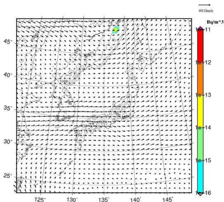
Xe-133 concentration at 3000m JST= 2017-09-06_18h00m
