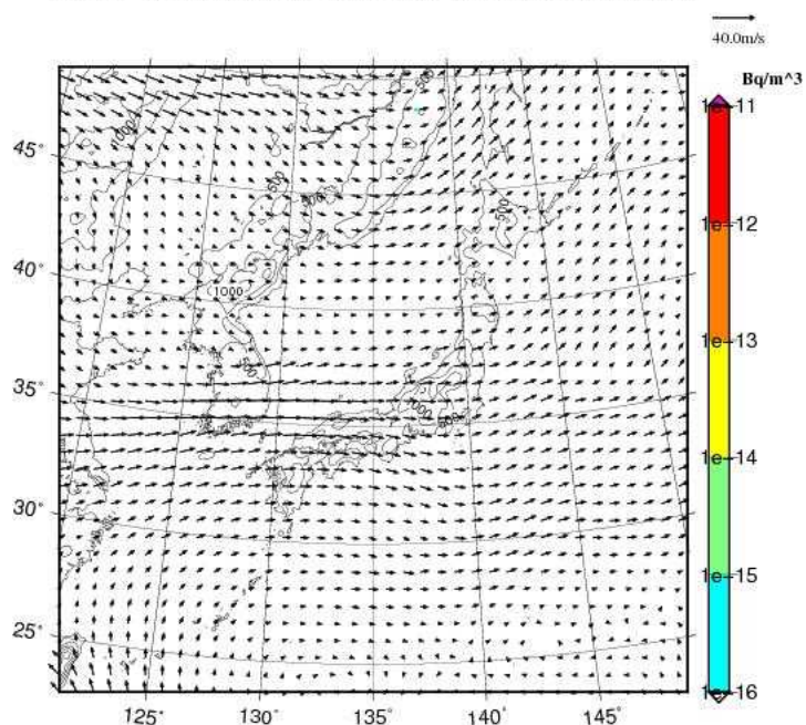
Cs-137 concentration at 3000m JST= 2017-09-06_18h00m
