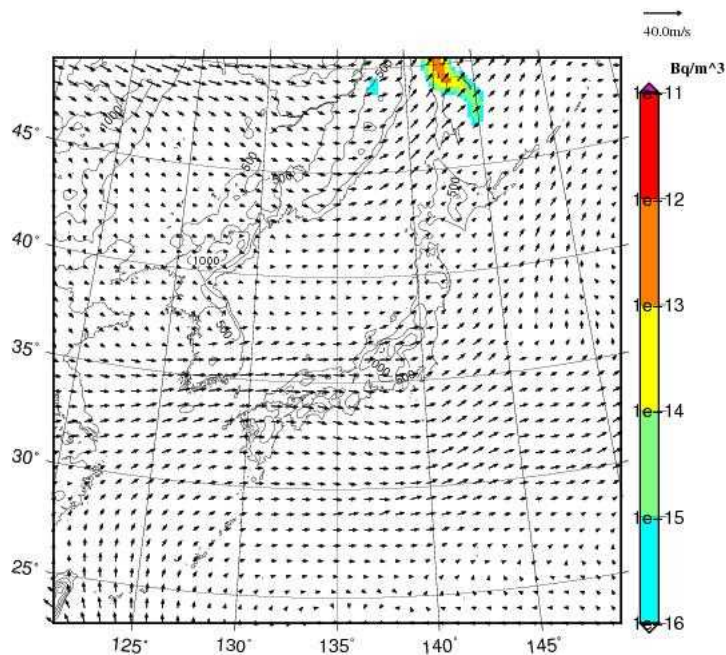
Cs-137 concentration at 2000m JST= 2017-09-06_18h00m
