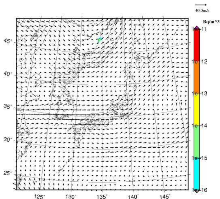
Xe-133 concentration at 3000m JST= 2017-09-06_09h00m
