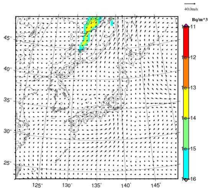
I-131 concentration at surface JST= 2017-09-06_09h00m
