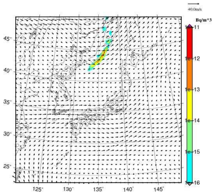
Cs-137 concentration at 2000m JST= 2017-09-06_15h00m
