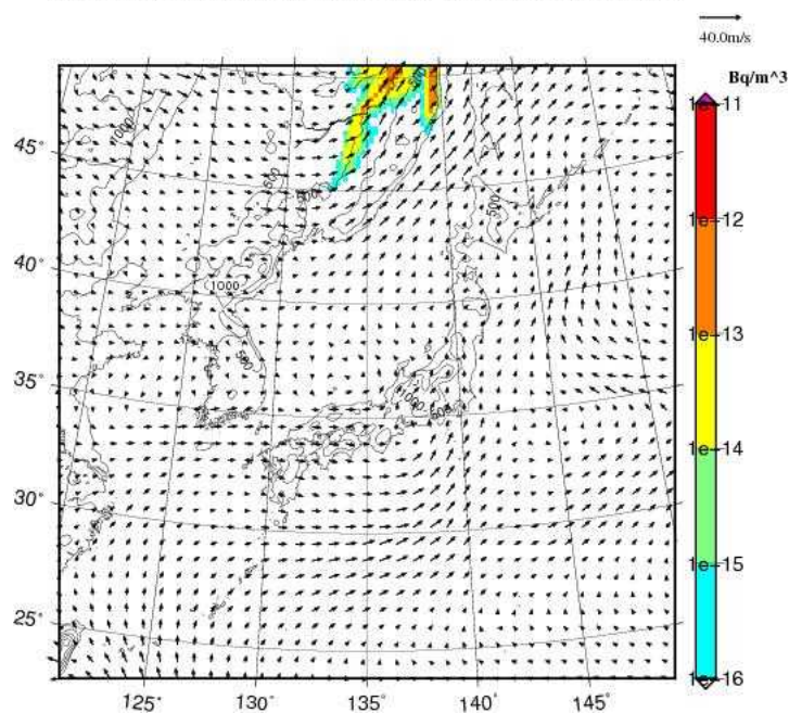
Xe-133 concentration at 1000m JST= 2017-09-06_09h00m
