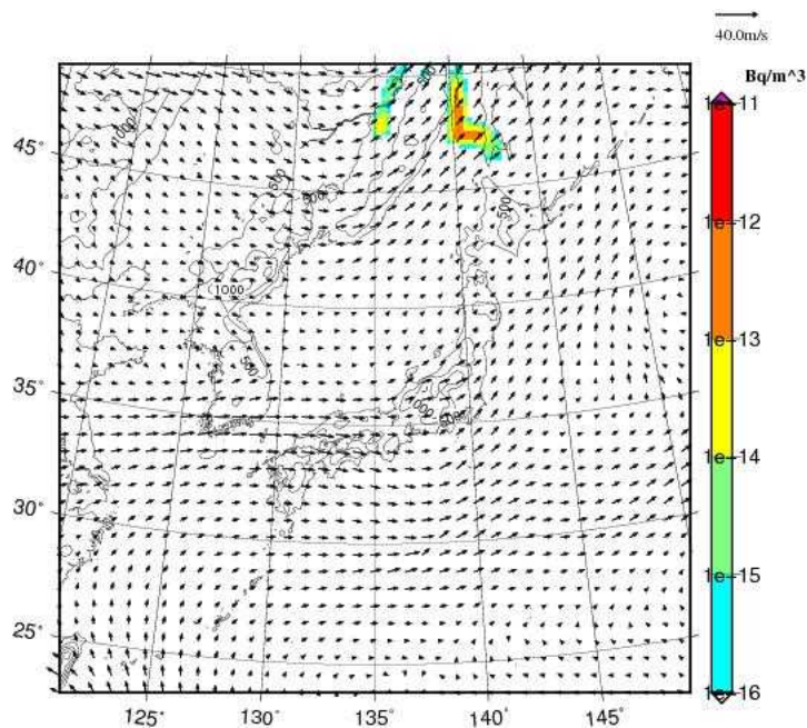
Xe-133 concentration at 2000m JST= 2017-09-06_12h00m
