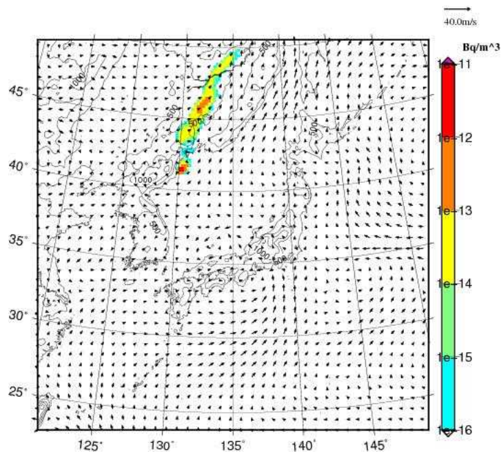
Xe-133 concentration at surface JST= 2017-09-06_09h00m
