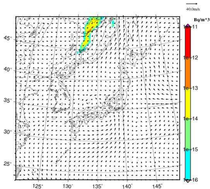
Cs-137 concentration at surface JST= 2017-09-06_09h00m
