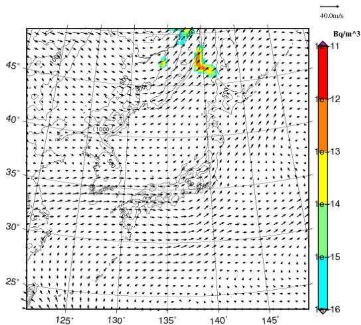
Xe-133 concentration at 2000m JST= 2017-09-06_09h00m
