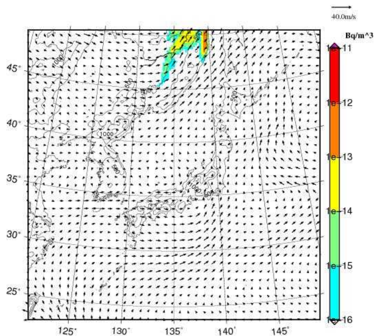
I-131 concentration at 1000m JST= 2017-09-06_09h00m
