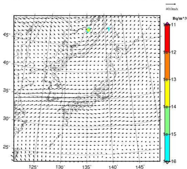
Xe-133 concentration at 3000m JST= 2017-09-06_12h00m
