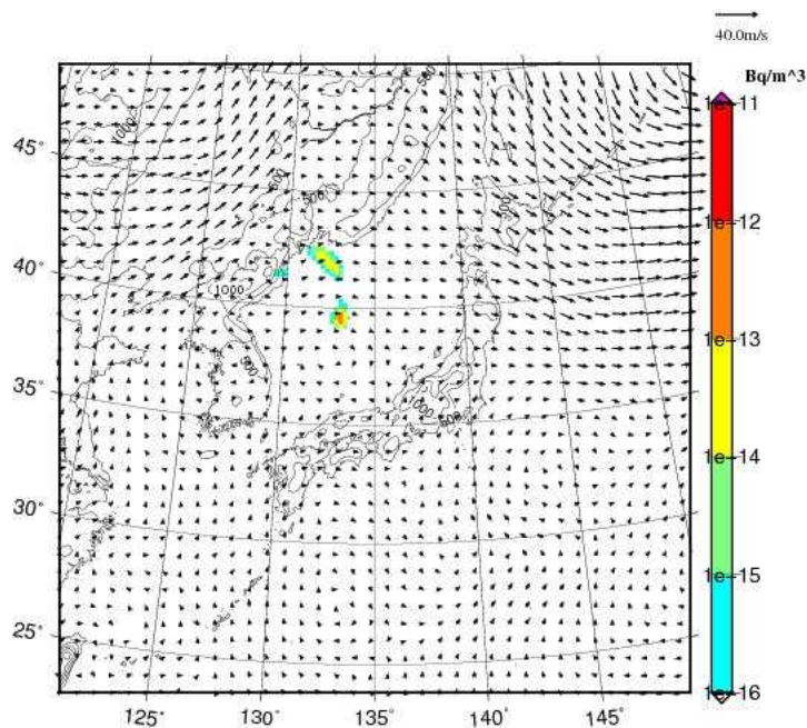
Cs-137 concentration at 2000m JST= 2017-09-04_15h00m
