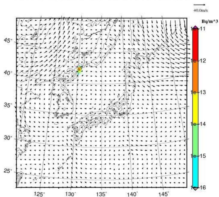
Cs-137 concentration at 1000m JST= 2017-09-04_09h00m
