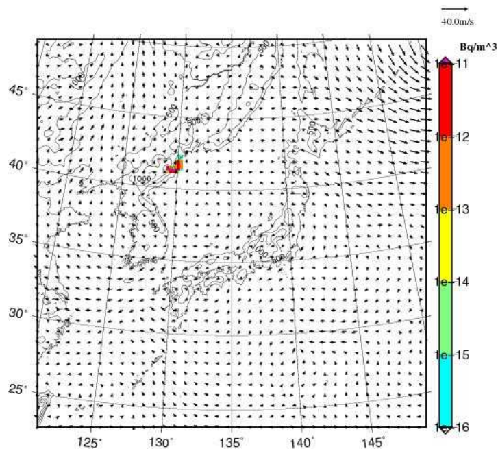
Xe-133 concentration at surface JST= 2017-09-04_09h00m
