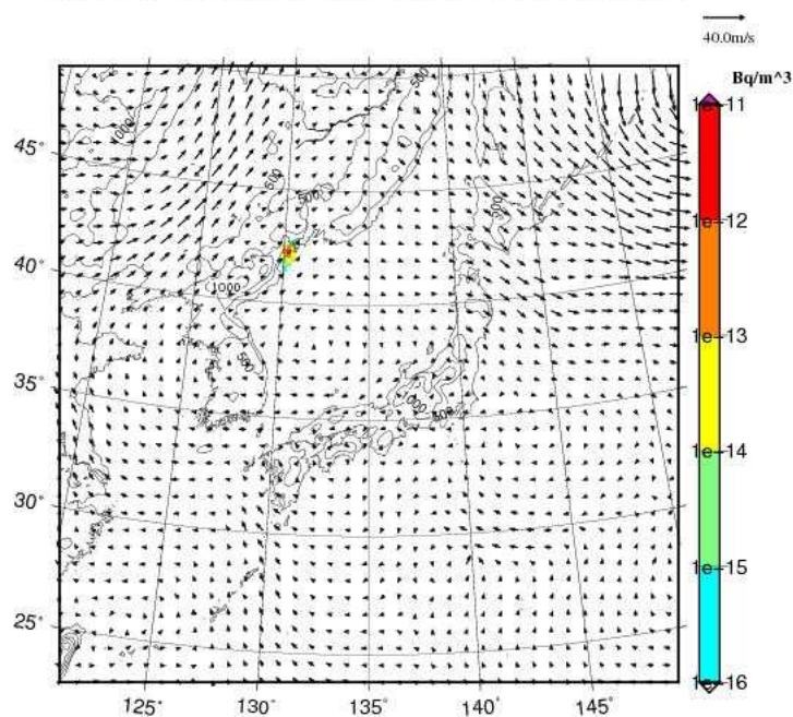
Xe-133 concentration at 1000m JST= 2017-09-04_09h00m
