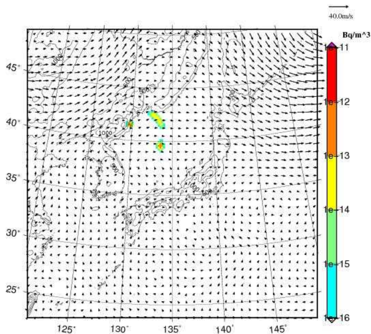
Cs-137 concentration at 2000m JST= 2017-09-04_18h00m
