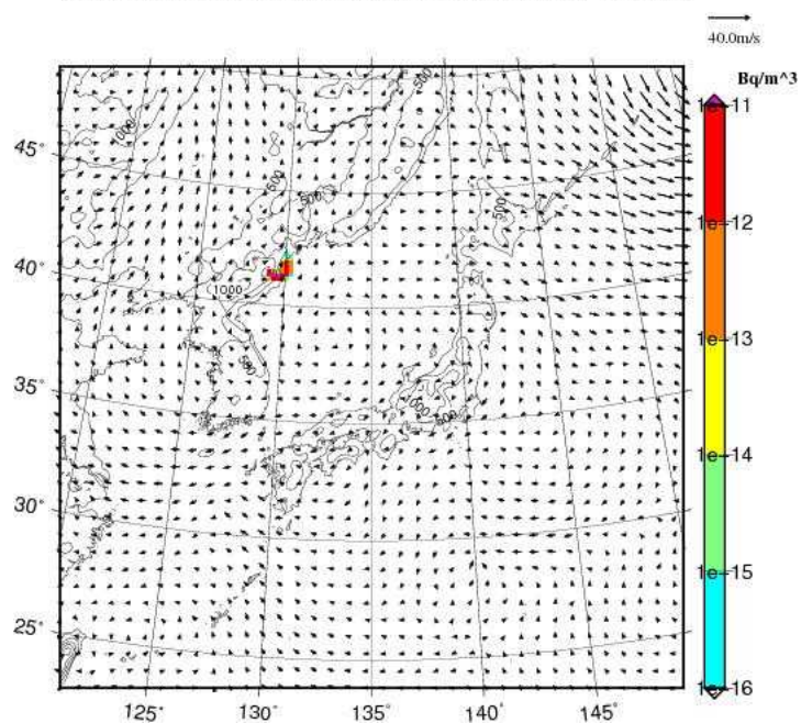
Cs-137 concentration at surface JST= 2017-09-04_09h00m
