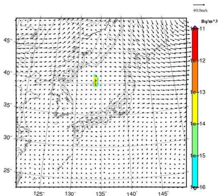
Cs-137 concentration at 3000m JST= 2017-09-04_18h00m
