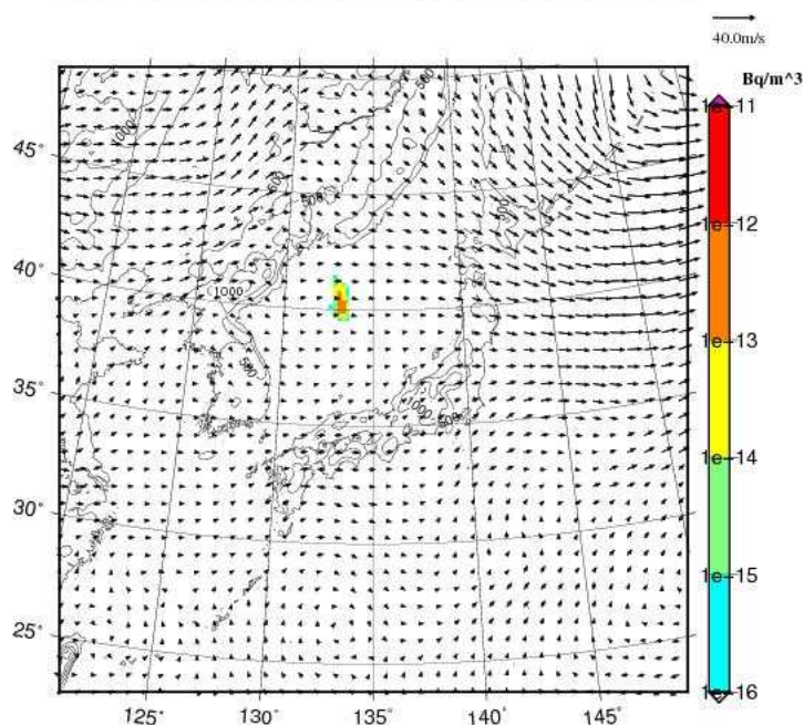
Cs-137 concentration at 3000m JST= 2017-09-04_15h00m
