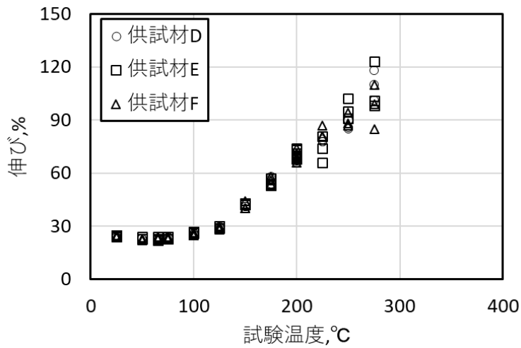
(c) 伸び
