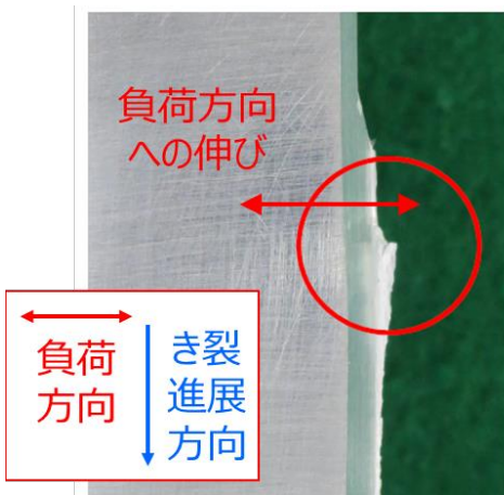
[破面の側面]
