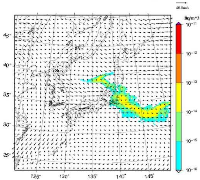
I-131 concentration at surface UTC= 2013-02-22_09h
