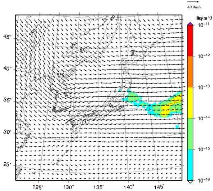
Xe-133 concentration at 2000m UTC= 2013-02-22_06h
