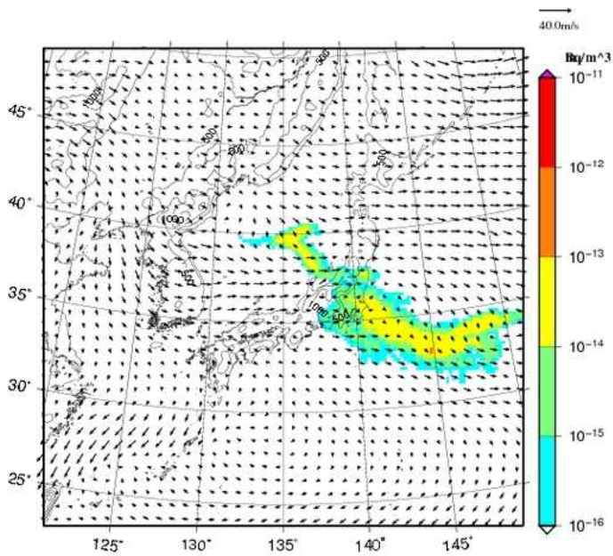
I-131 concentration at surface UTC= 2013-02-22_06h
