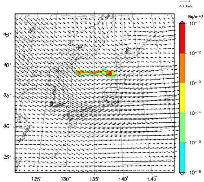
Cs-137 concentration at 1000m UTC= 2013-02-22_06h
