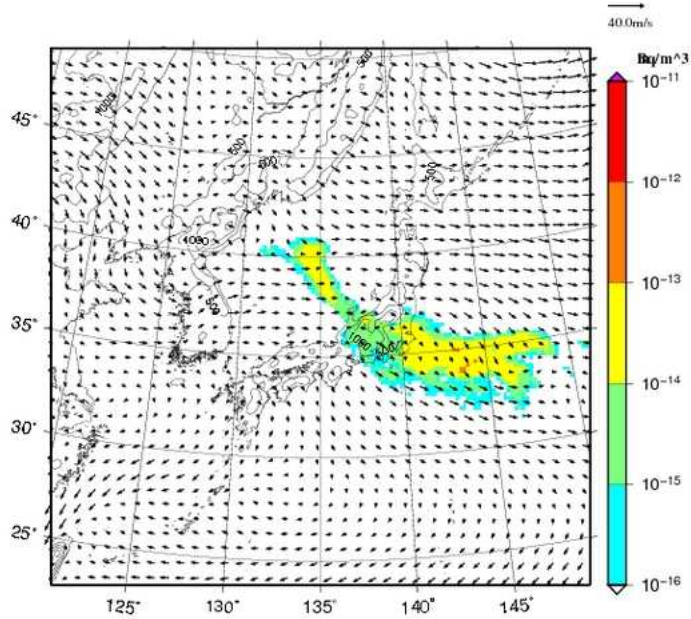
I-131 concentration at surface UTC= 2013-02-22_00h
