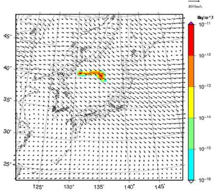
I-131 concentration at 1000m UTC= 2013-02-22_00h
