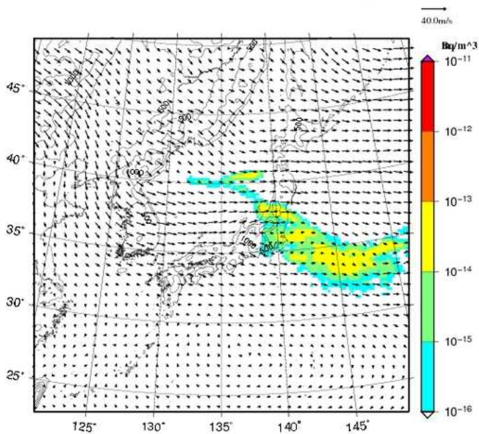
I-131 concentration at 1000m UTC= 2013-02-22_06h
