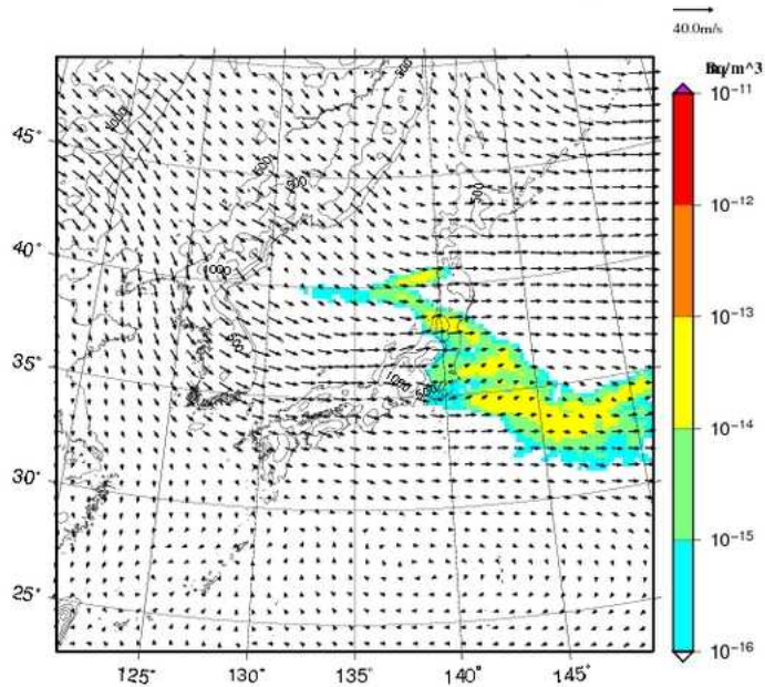
I-131 concentration at 1000m UTC= 2013-02-22_09h
