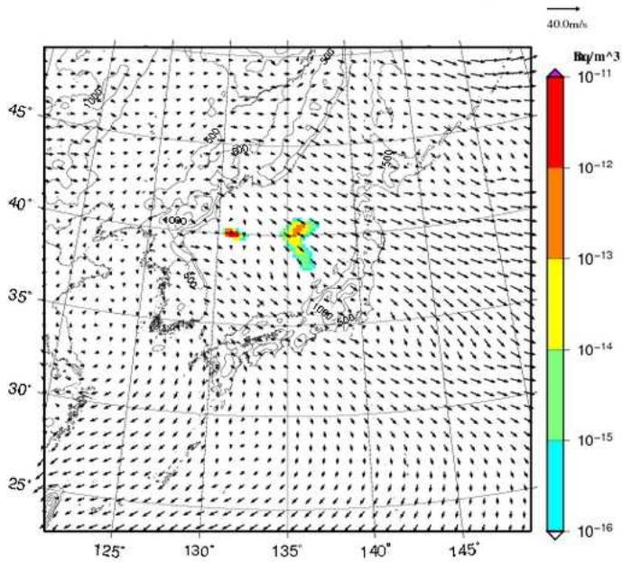
Xe-133 concentration at surface UTC= 2013-02-22_03h
