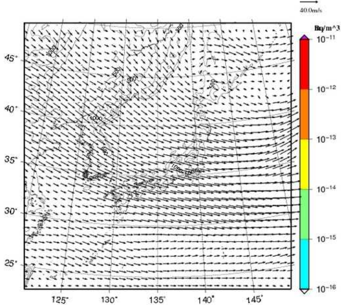
I-131 concentration at 3000m UTC= 2013-02-22_00h
