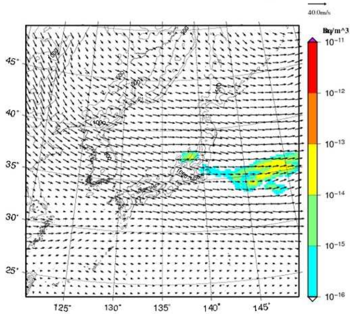
I-131 concentration at 2000m UTC= 2013-02-22_00h
