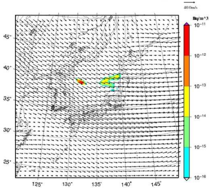
Cs-137 concentration at surface UTC= 2013-02-22_09h
