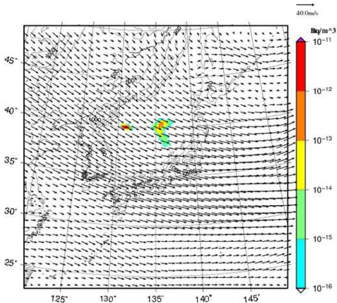
Cs-137 concentration at surface UTC= 2013-02-22_03h
