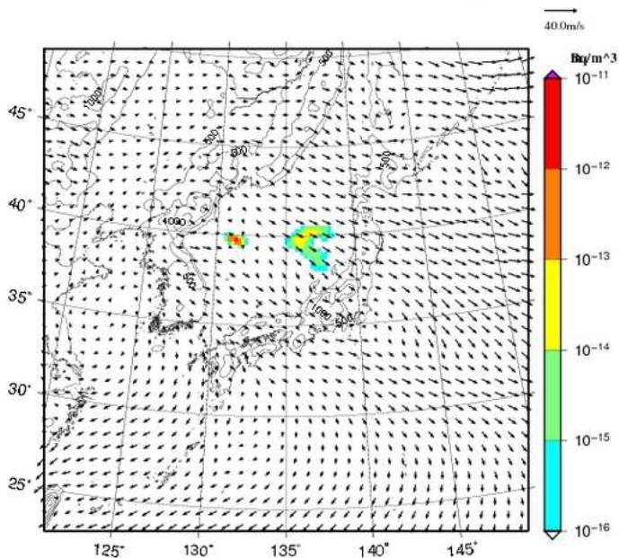
I-131 concentration at surface UTC= 2013-02-22_06h
