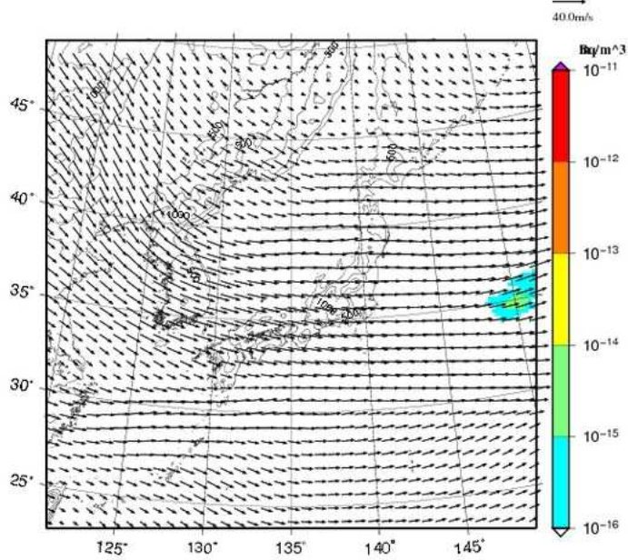
Xe-133 concentration at 3000m UTC= 2013-02-22_06h
