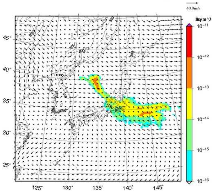
Xe-133 concentration at surface UTC= 2013-02-22_00h
