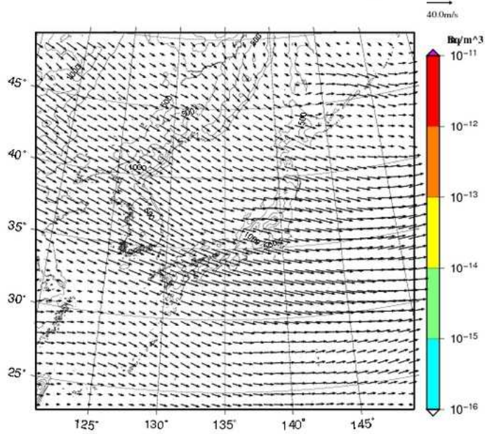
I-131 concentration at 3000m UTC= 2013-02-22_06h
