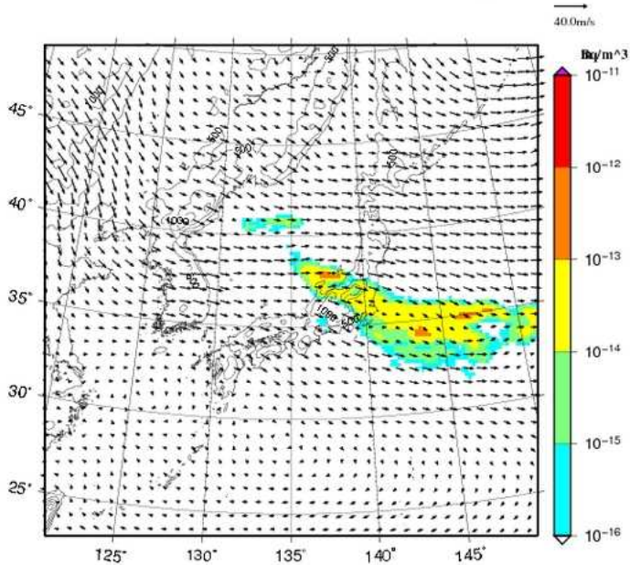
Xe-133 concentration at 1000m UTC= 2013-02-22_00h
