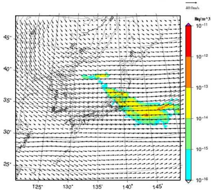
Cs-137 concentration at 1000m UTC= 2013-02-22_03h
