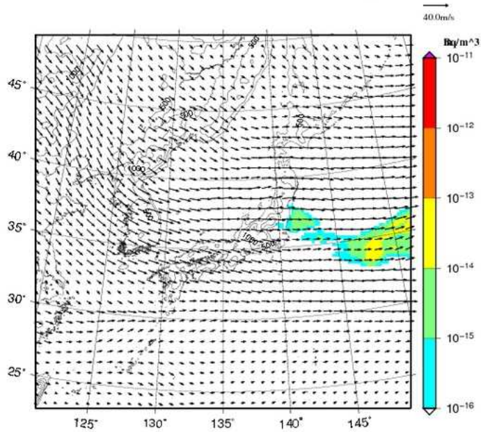
I-131 concentration at 2000m UTC= 2013-02-22_06h
