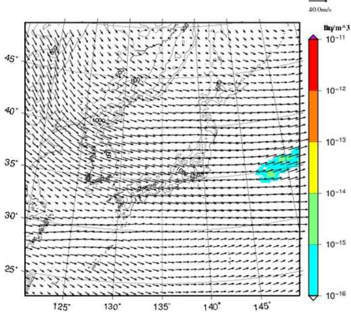
Cs-137 concentration at 3000m UTC= 2013-02-22_03h
