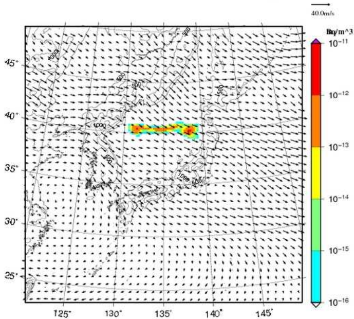
I-131 concentration at 1000m UTC= 2013-02-22_06h
