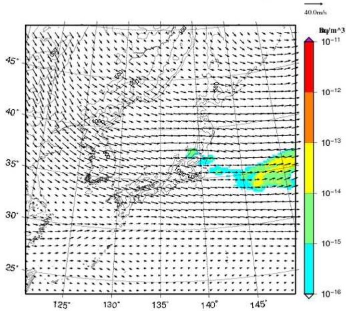
I-131 concentration at 2000m UTC= 2013-02-22_03h
