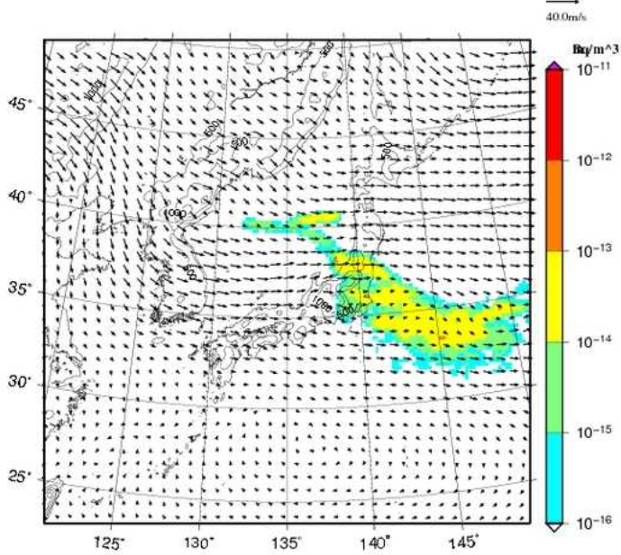
Xe-133 concentration at 1000m UTC= 2013-02-22_06h
