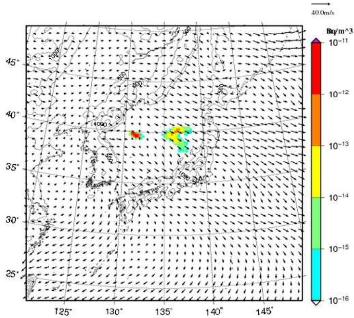
Xe-133 concentration at surface UTC= 2013-02-22_06h
