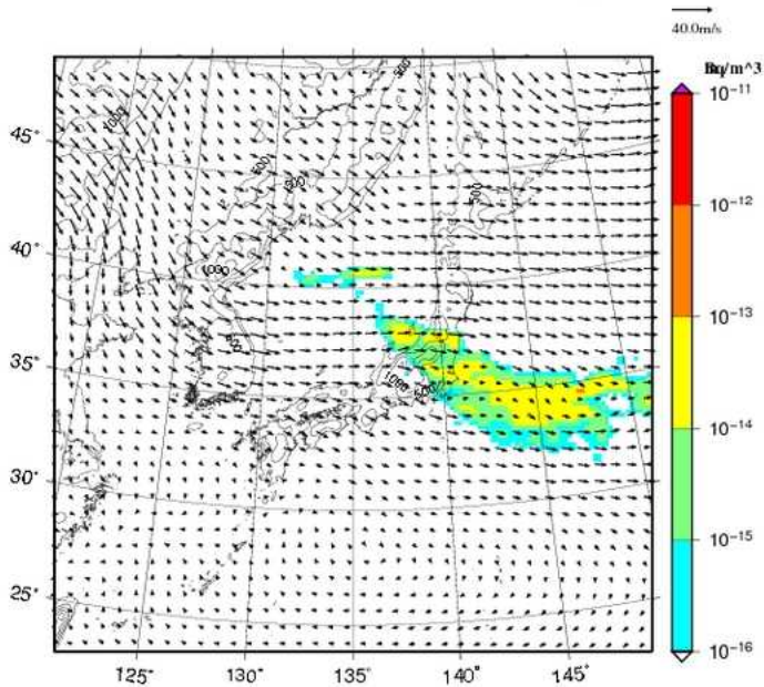
I-131 concentration at 1000m UTC= 2013-02-22_03h
