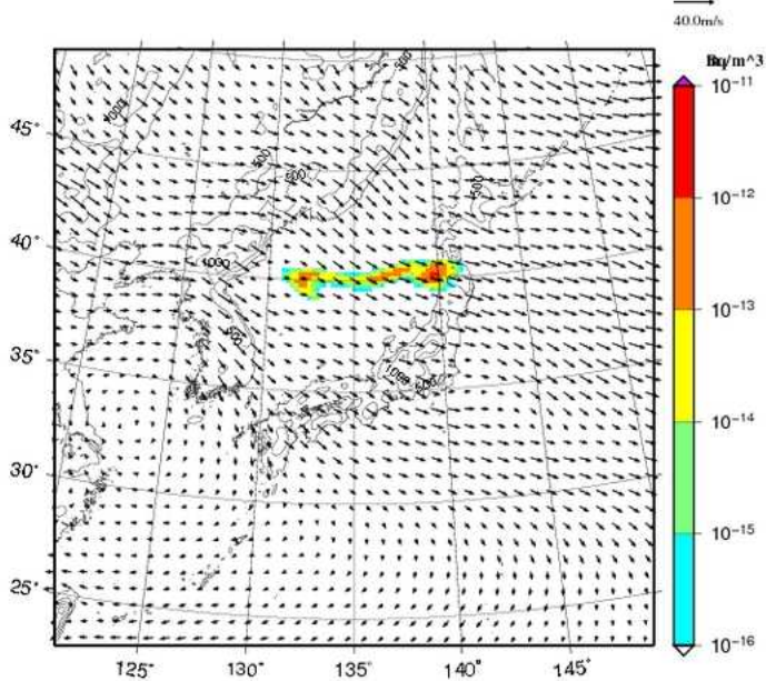
Xe-133 concentration at 1000m UTC= 2013-02-22_09h
