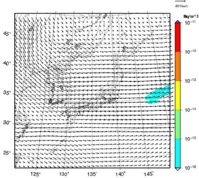
I-131 concentration at 3000m UTC= 2013-02-22_03h
