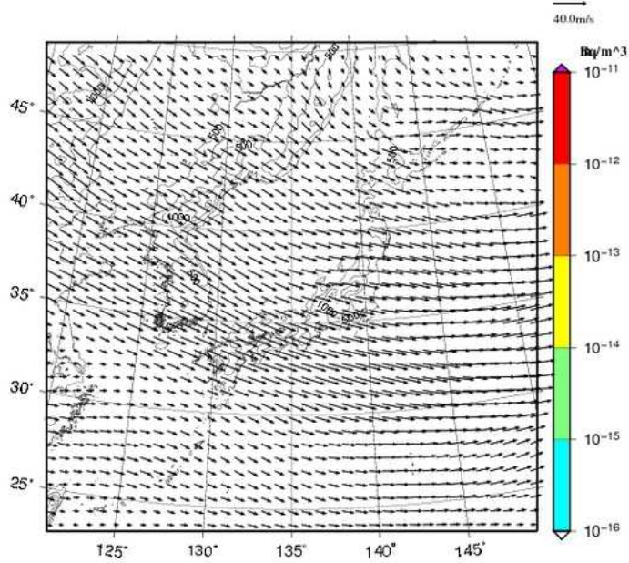
I-131 concentration at 3000m UTC= 2013-02-22_09h
