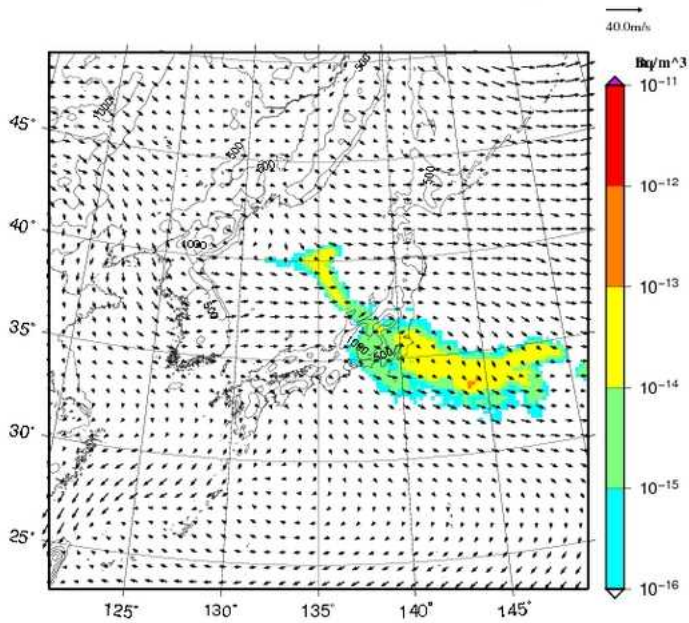
I-131 concentration at surface UTC= 2013-02-22_03h
