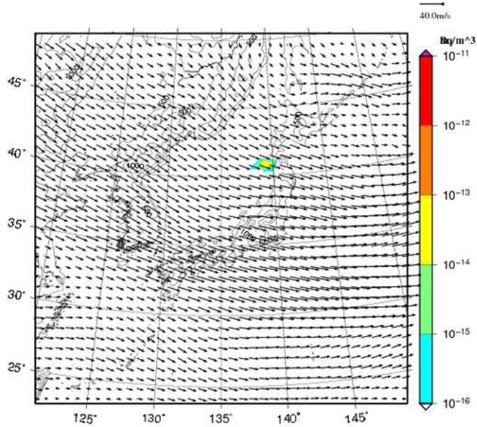
Cs-137 concentration at 2000m UTC= 2013-02-22_06h
