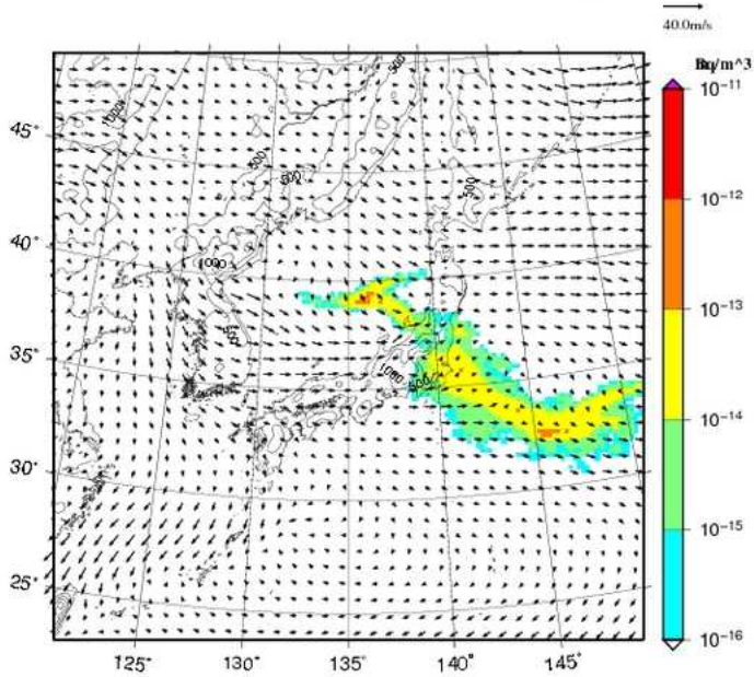
Xe-133 concentration at surface UTC= 2013-02-22_09h
