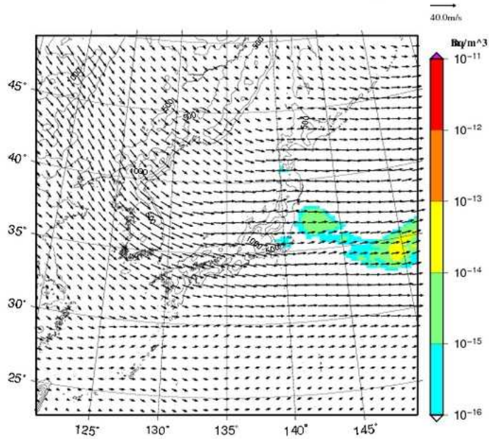
I-131 concentration at 2000m UTC= 2013-02-22_09h
