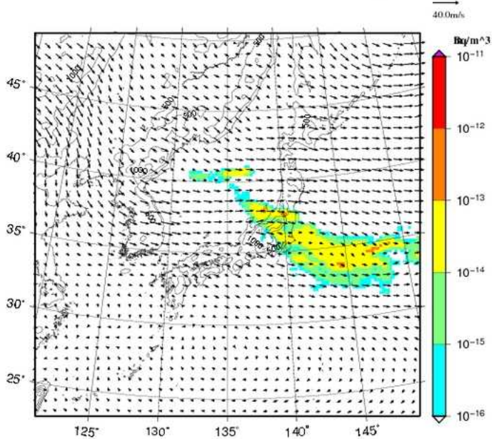
Xe-133 concentration at 1000m UTC= 2013-02-22_03h
