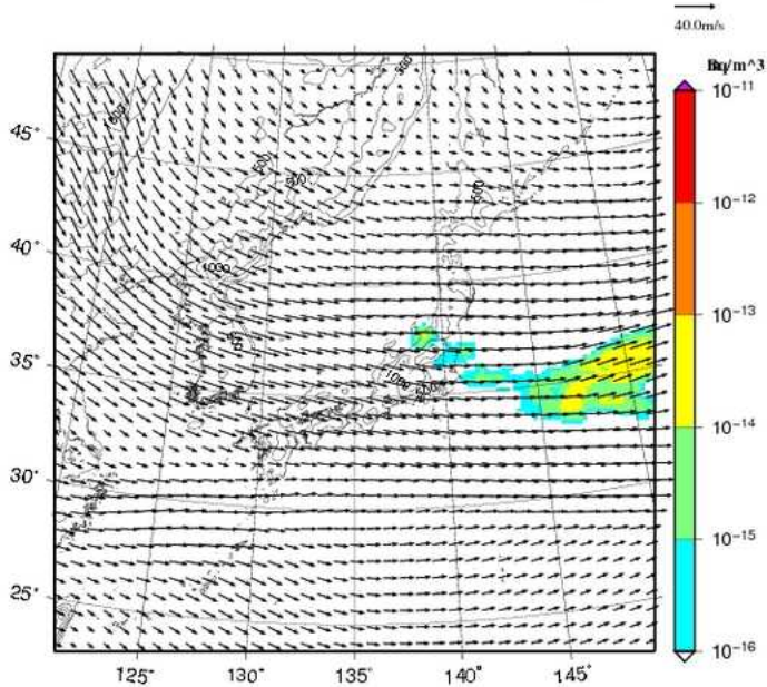
Cs-137 concentration at 2000m UTC= 2013-02-22_03h
