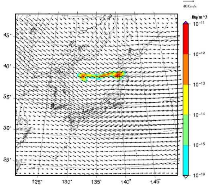
Cs-137 concentration at 1000m UTC= 2013-02-22_09h
