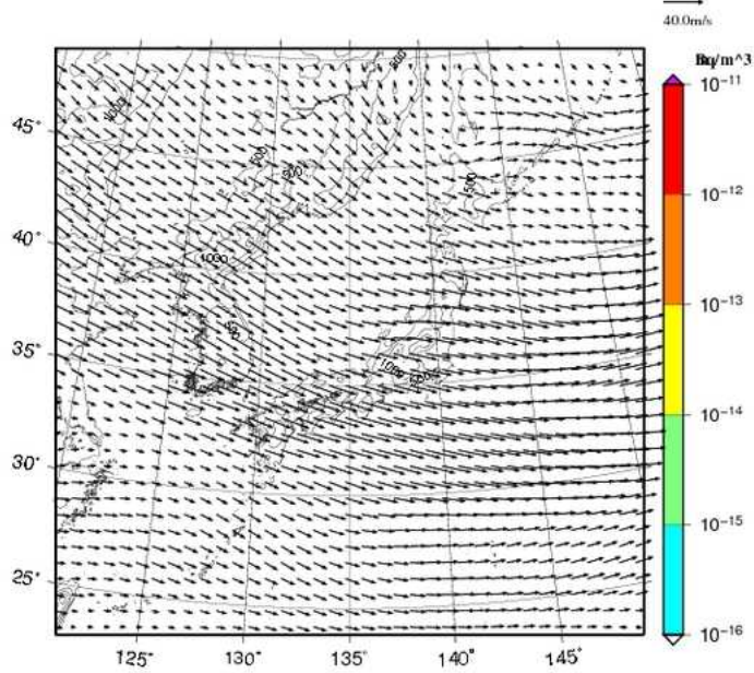
Cs-137 concentration at 3000m UTC= 2013-02-22_06h
