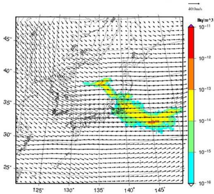
Cs-137 concentration at surface UTC= 2013-02-22_06h
