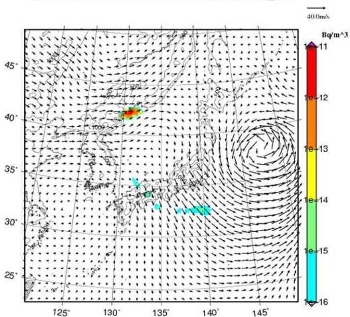
Xe-133 concentration at 1000m UTC= 2013-02-13_09h
