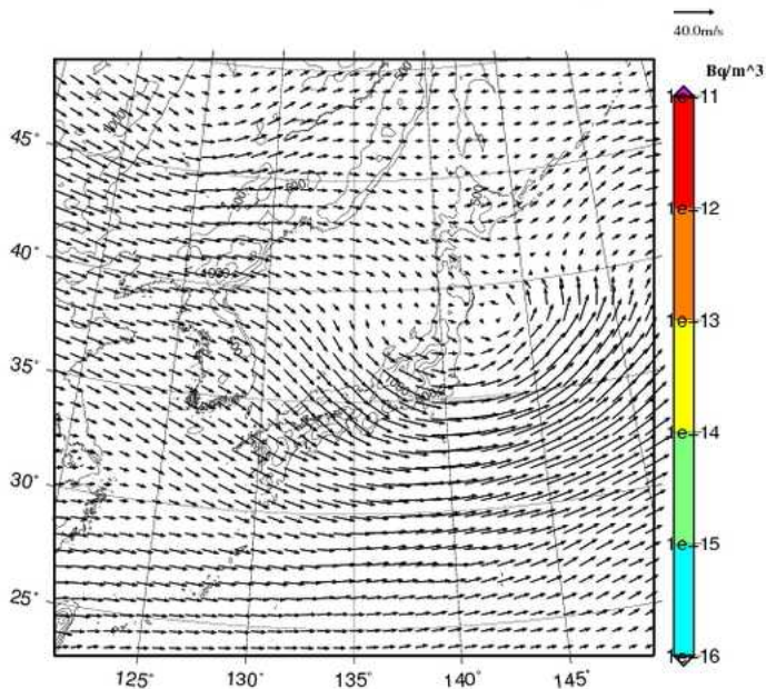
Xe-133 concentration at 3000m UTC= 2013-02-13_03h
