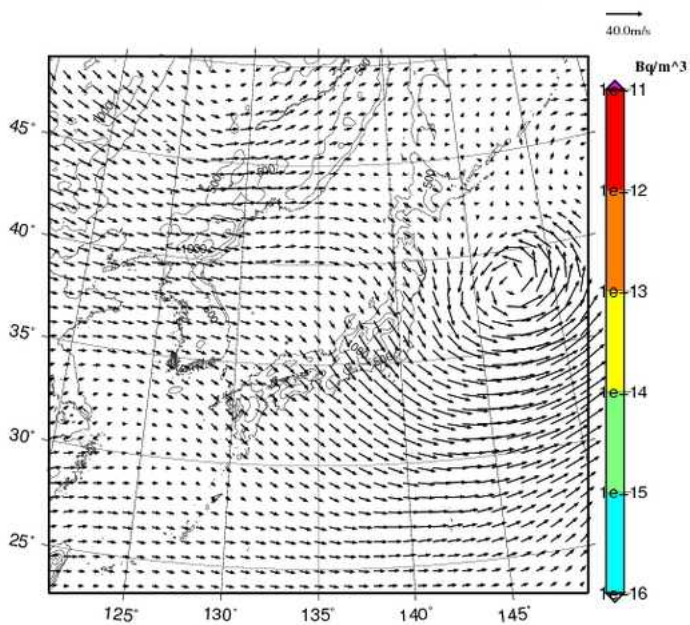
Xe-133 concentration at 2000m UTC= 2013-02-13_09h
