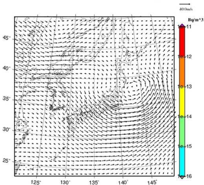
Xe-133 concentration at 2000m UTC= 2013-02-13_03h
