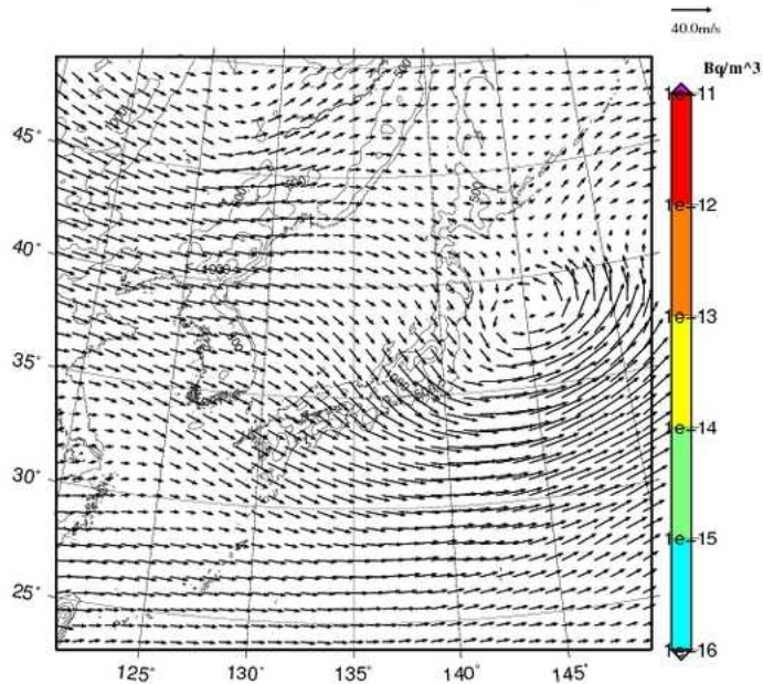
Xe-133 concentration at 3000m UTC= 2013-02-13_06h
