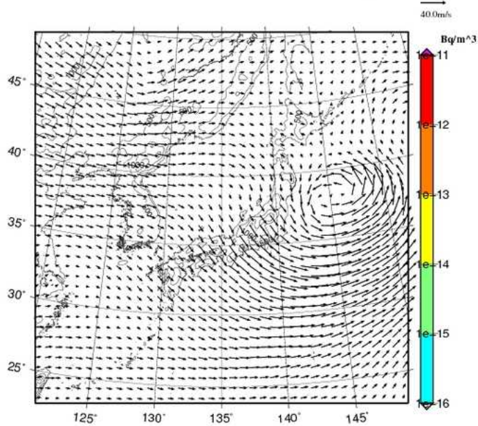
Xe-133 concentration at 2000m UTC= 2013-02-13_06h
