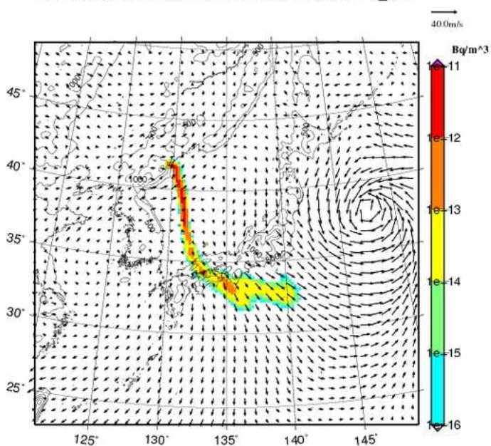
Xe-133 concentration at surface UTC= 2013-02-13_09h
