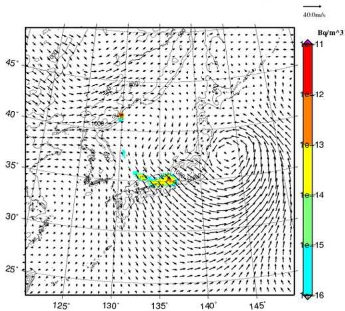
Xe-133 concentration at 1000m UTC= 2013-02-13_03h
