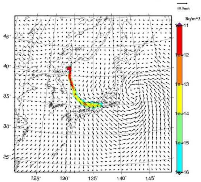
Xe-133 concentration at surface UTC= 2013-02-13_03h
