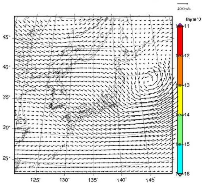
Xe-133 concentration at 3000m UTC= 2013-02-13_09h
